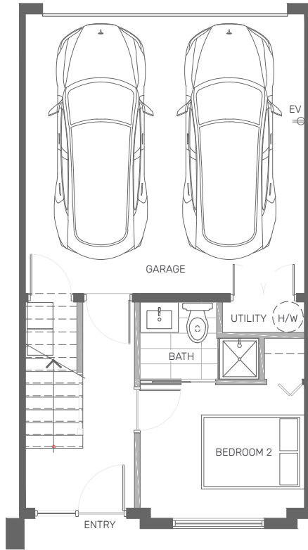
LEVEL 1 1ST FLOOR
