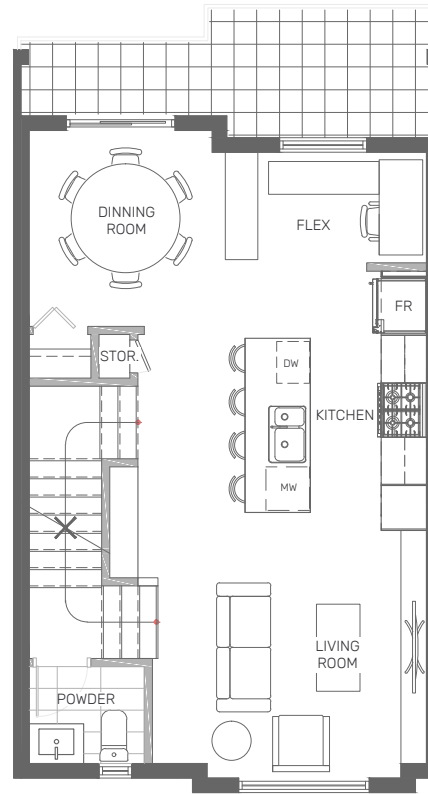
LEVEL 2 2ND FLOOR
